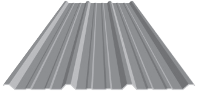
Panel Coverage: 36" wide Rib Height: 1-1/4" Available Lengths: 10', 12', 16', 20' & 24' Rib Feature: Trapezoidal Rib on 12" Centers Material: Steel Fasteners: Exposed Standard Finish: Galvalume®
